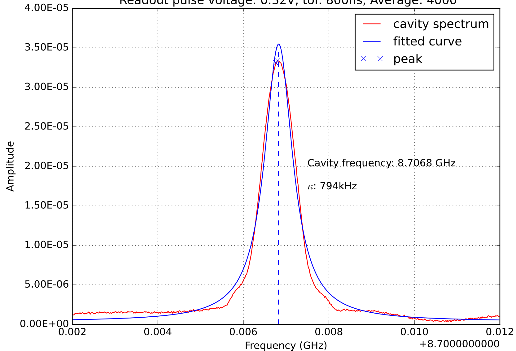
Readout cavity spectrum Readout pulse voltage: 0.32V, tof: 800ns, Average: 4000
